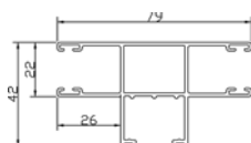
DF A15-H
